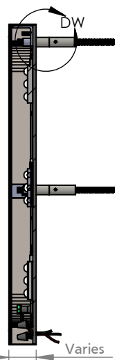
SECTION A-A II SCALE 1:5
