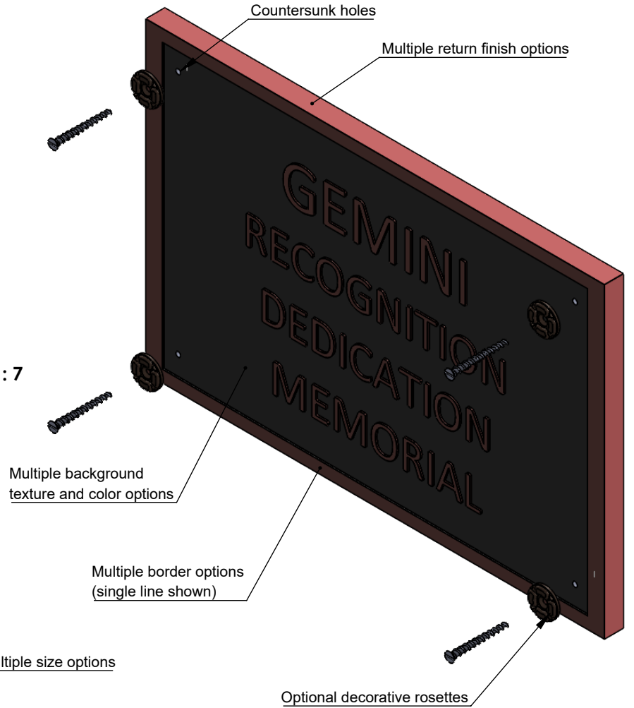
ISOMETRIC FRONT VIEW II SCALE 1 : 5
