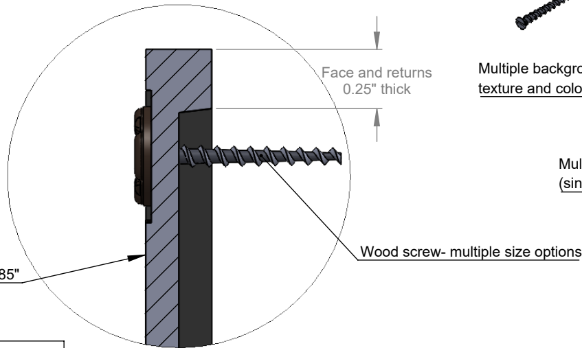
DETAIL DW SCALE 1 : 2
