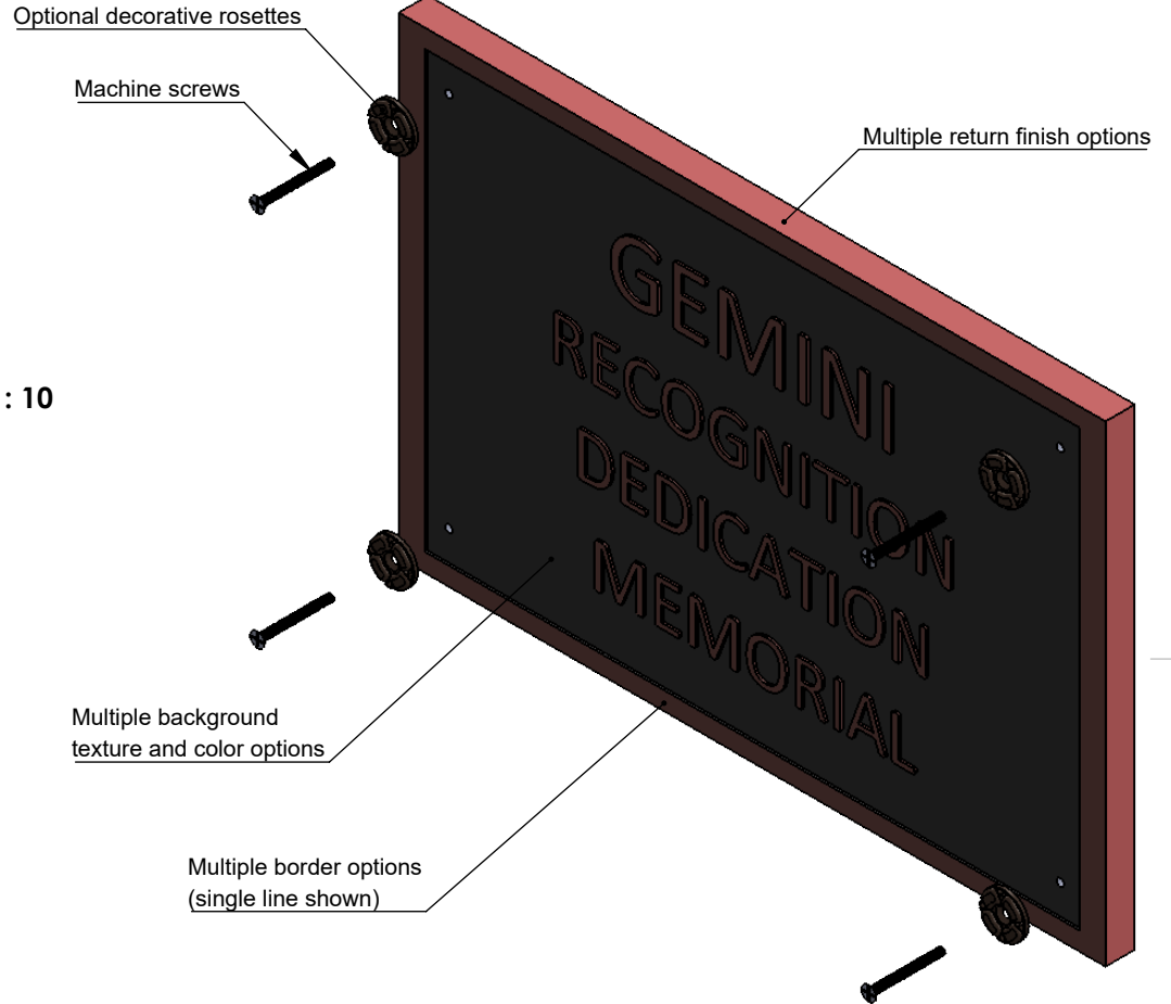
ISOMETRIC FRONT VIEW II SCALE 1 : 5
